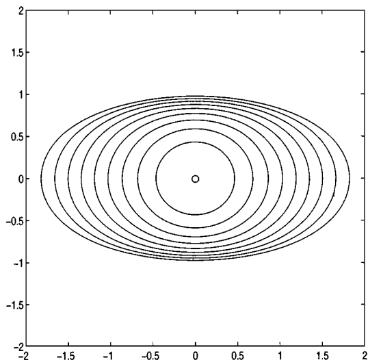
FIG. 8. N = 256 , \Delta t = 0.0025 , t = 0.0, 1.0(0.1) .
